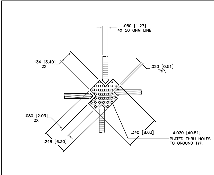
SUGGESTED TEST BOARD MOUNTING
